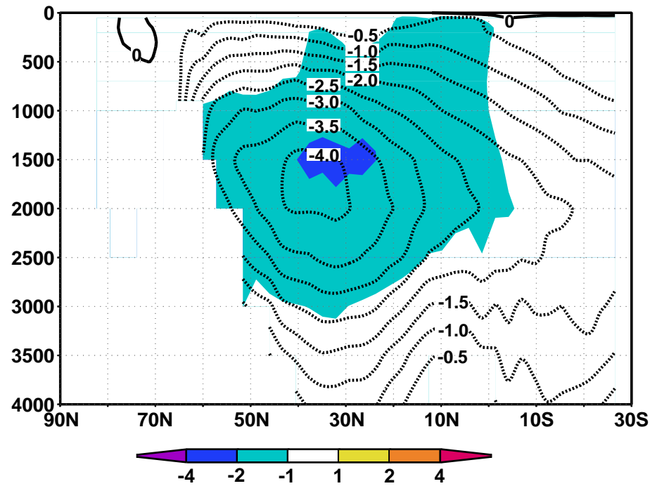
Atlantic Overturning Streamfunction (1000m)
