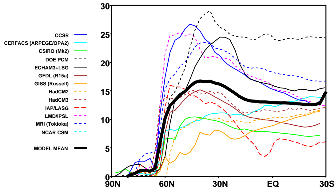
Atlantic Overturning Streamfunction (1000m)
