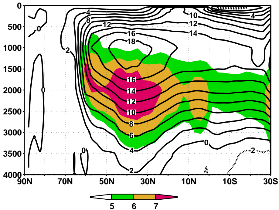
Atlantic Overturning Streamfunction Model Mean Contoured Model Standard Deviation Shaded
